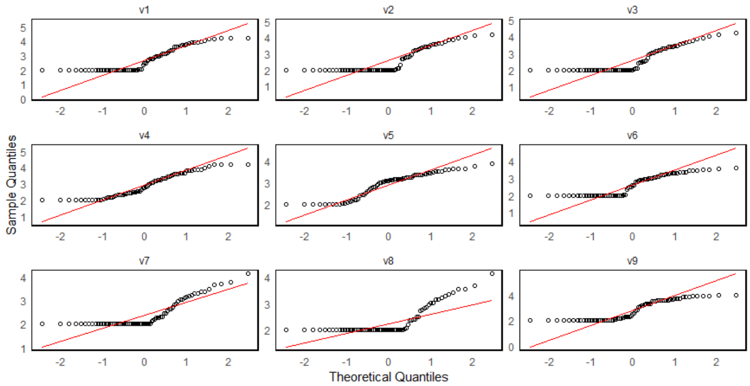
Q-Q Plots for v1 to v9
