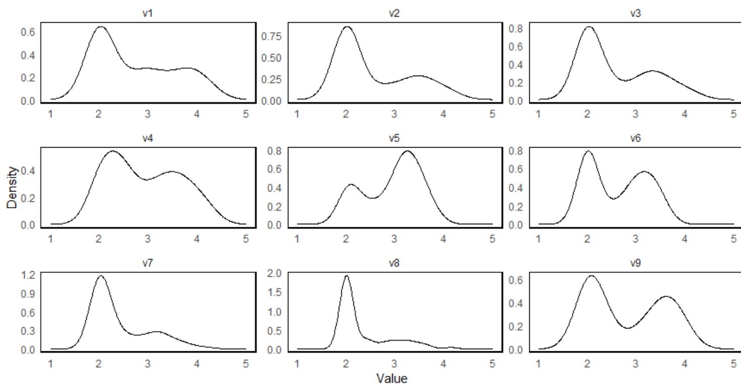
Density Plots of v1 to v9
